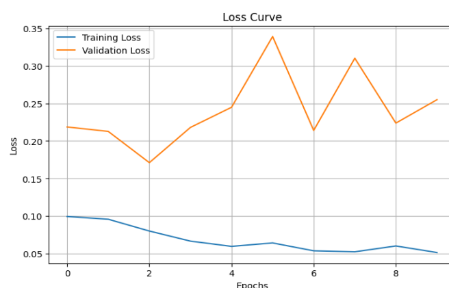
Figure. 4 Training and Validation Loss Curve
