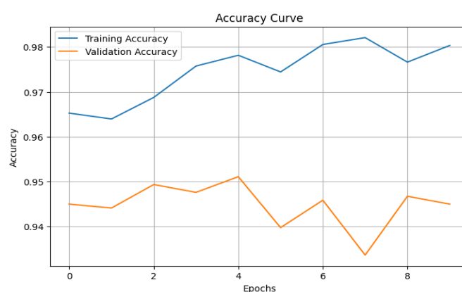
Figure. 3 Training and Validation Accuracy Curve
