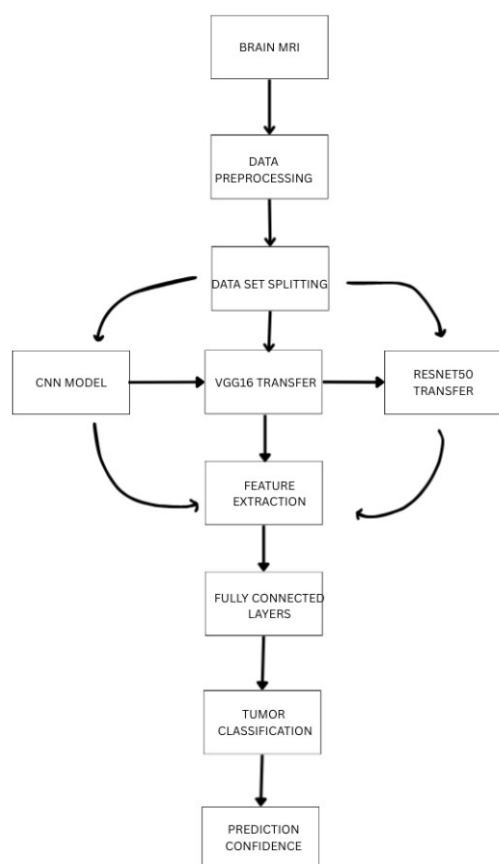
Figure.1 Flowchart of the Proposed Brain Tumor Classification System
