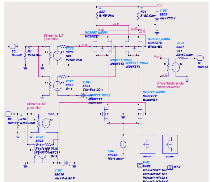
Figure 5. Gilbert cell mixer schematic in ADS using 130 nm CMOS model files
