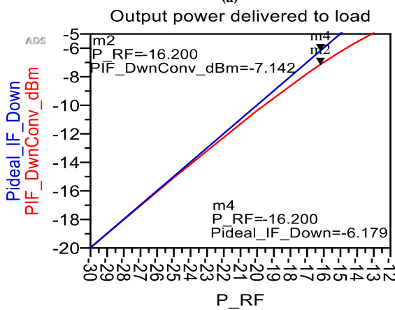
Figure. 6 Mixer Simulation
