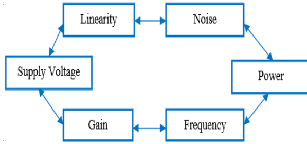
Figure 1. RF design trade-offs - Hexagon [1]
