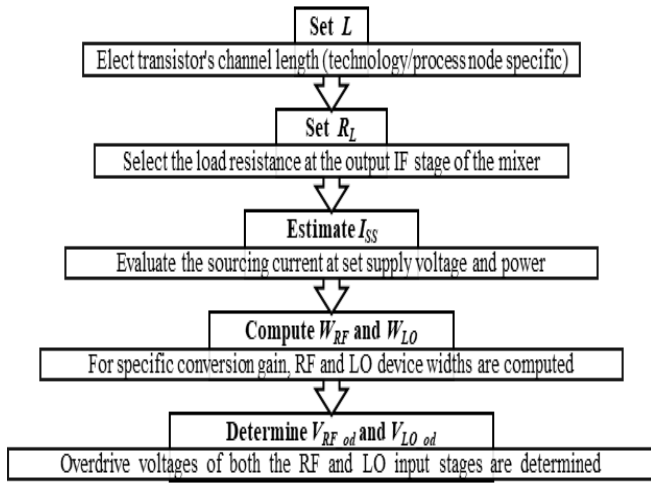
Figure 4. Design flow of the conventional mixer
