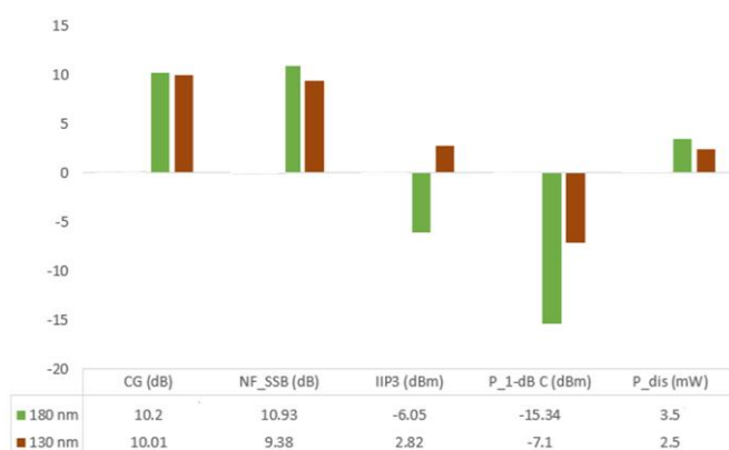
Figure 8. Visualization of mixer performance in various CMOS process nodes
