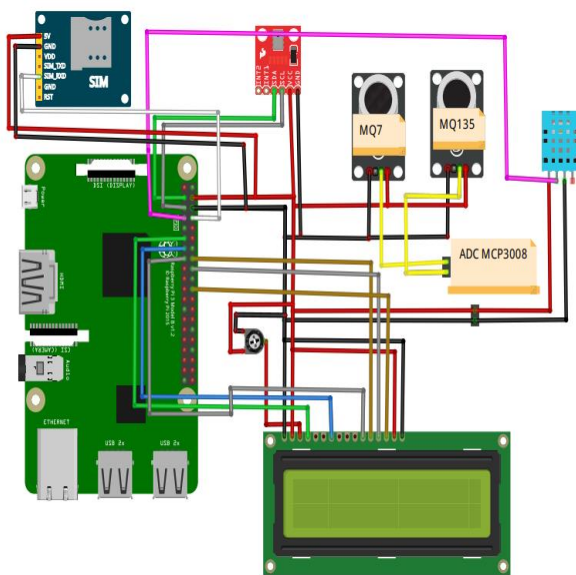
Fig 4.2 Circuit Diagram
