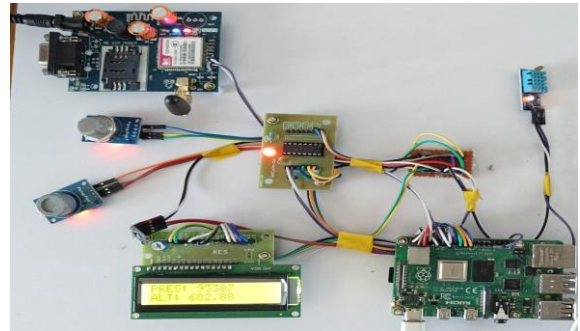
Fig 5.1 Showing results of Pressure and Alt
