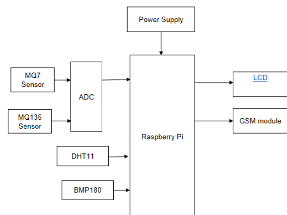
Fig 4.1 Block Diagram.
