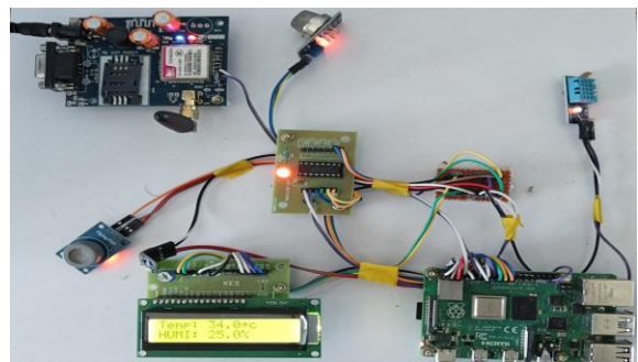
Fig 5.2 Showing results of Temperature and Humidity
