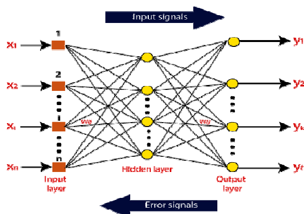
Fig.2 ANN
