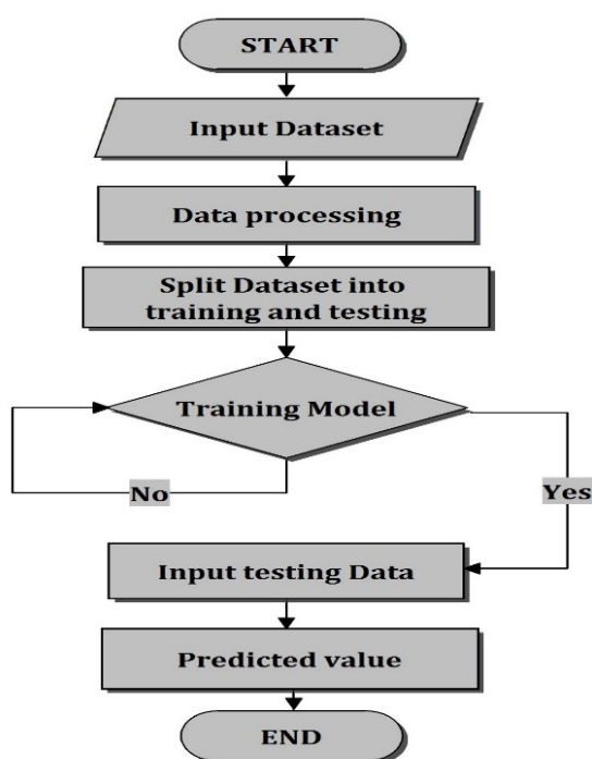
Fig.3 Flow Chart
