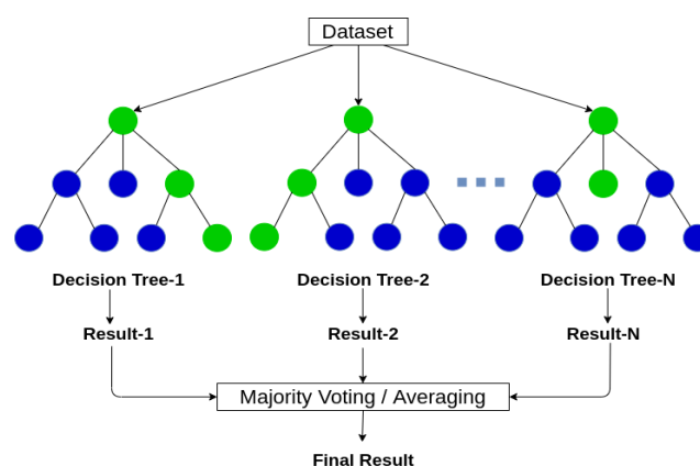
Fig.1 Random Forest
