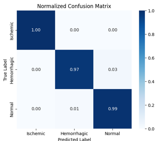
Fig.5 Confusion matrix of the proposed model
