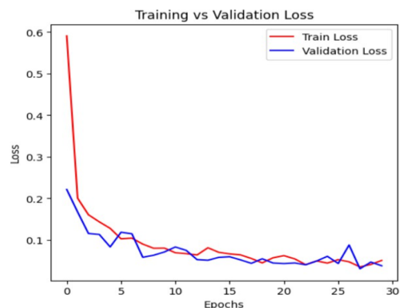
Fig. 4. Loss graph of the proposed model
