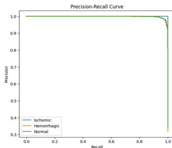
Fig.7 Precision-Recall Curve (PRC) of the proposed model
