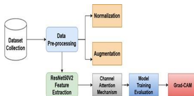
Fig.1. Architecture Diagram of the Proposed Model
