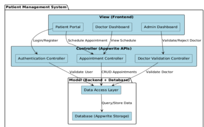
Figure.1 Over View of PMS Work Flow
