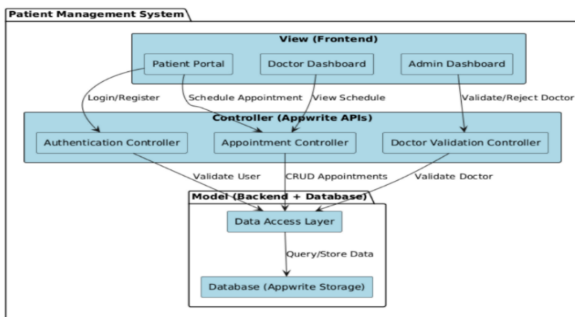
Figure.1 Over View of PMS Work Flow
