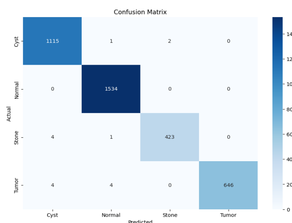
Fig.7 Confusion matrix illustrating per-class classification results.
