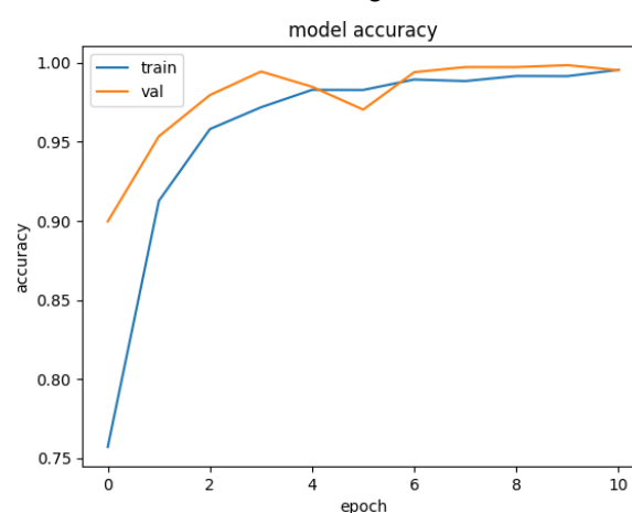
Fig. 5 Training and validation accuracy curve over epochs.
