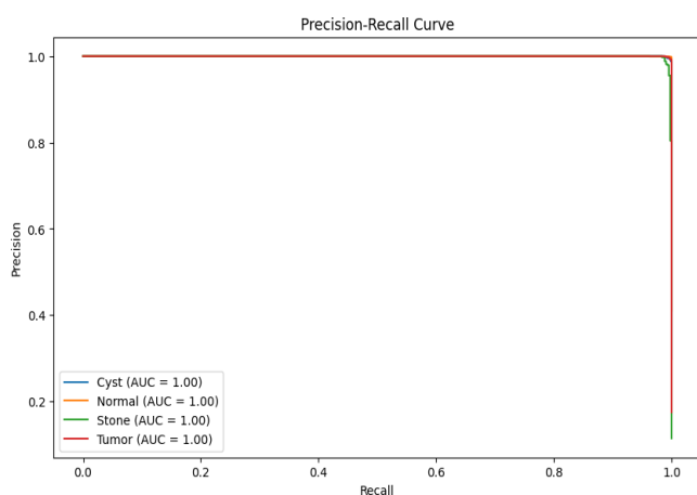
Fig.3. Precision-Recall Curve (PRC) showing the trade-off between precision and recall for each class.
