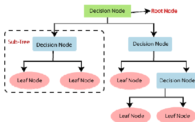
Figure.3 Decision-Tree approach
